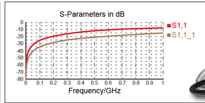
Return Loss
