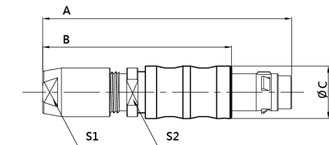
Standard back nut with bend relief
