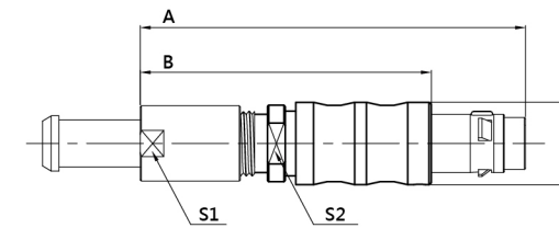
Standard back nut
