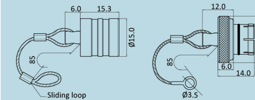
PLUG PROTECTIVE CAP SOCKET PROTECTIVE CAP
