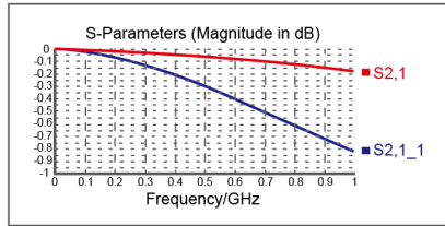
Insertion Loss
